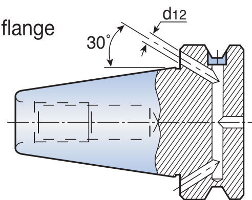
Type “ADB” Coolant hole or coolant through flange
