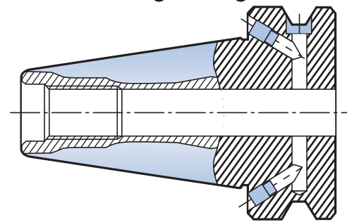
Type “ADB” Coolant hole or coolant through flange
